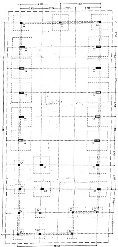
CENTER LINE PLAN
